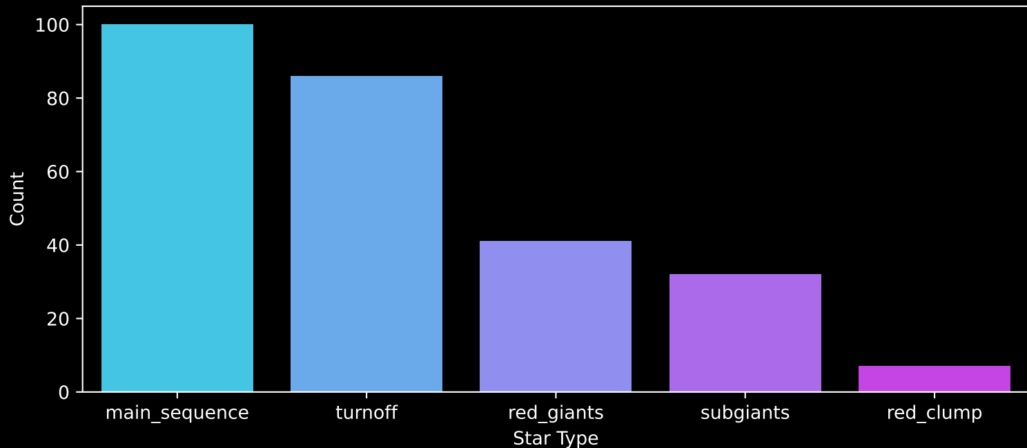
GALAH DR4 Field: [1646] Count plot of Star Type
