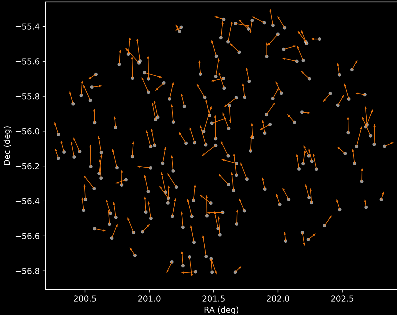
GALAH DR4 Cluster 2 Proper Motion Vectors (n=165)
