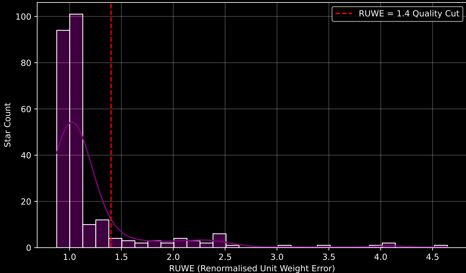
GALAH DR4 Field [1646] RUWE Distribution (n= 253)
